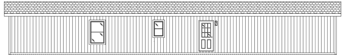
REAR SIDEWALL
